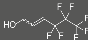
Allylic 3:3 FTOH
